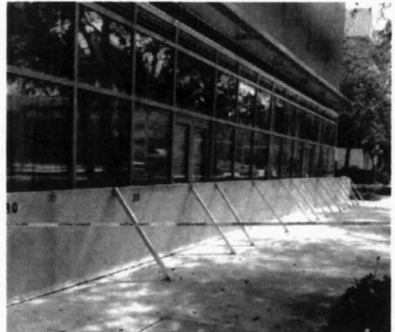
Use of flood barriers to protect building from flood damage on Pennsylvania Ave. Miami Beach. Source: Miami Beach
