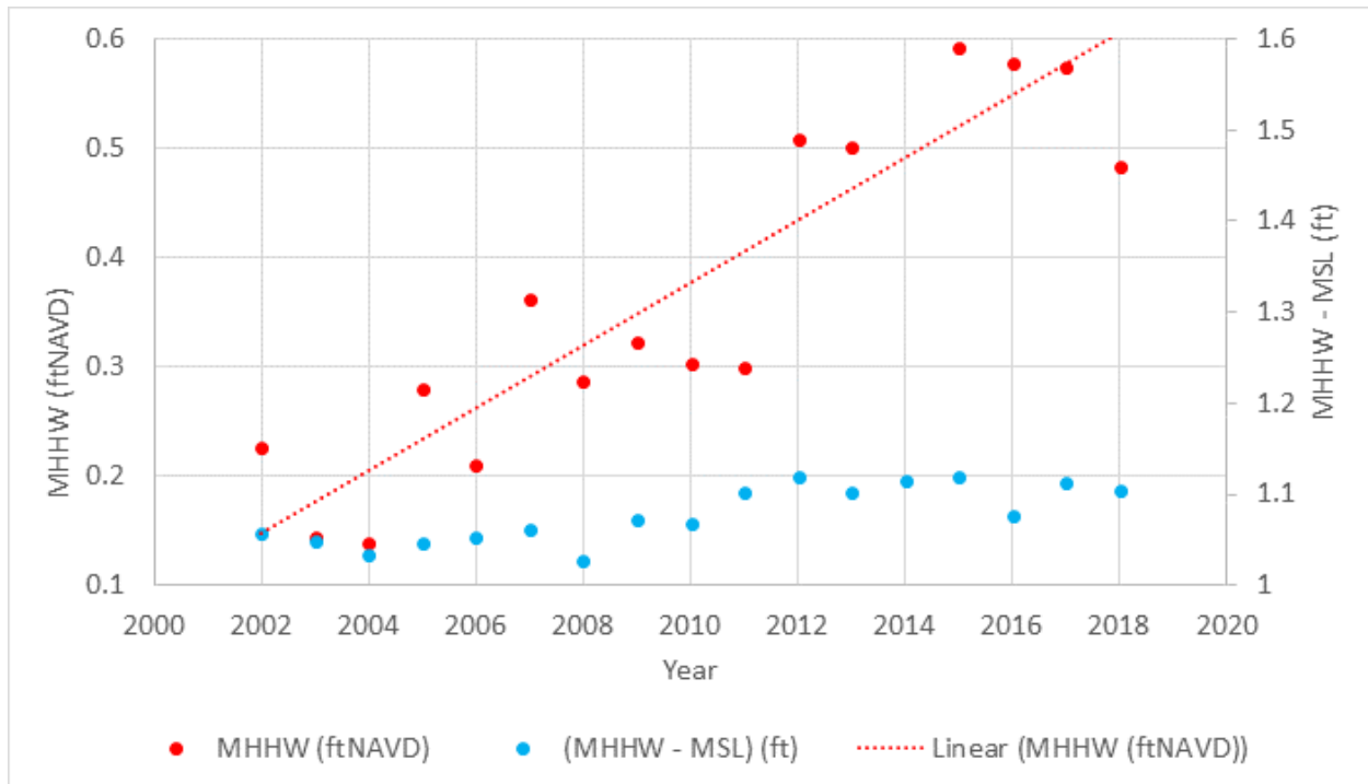
Figure C-2. Variation of MHHW over time, Second Method
