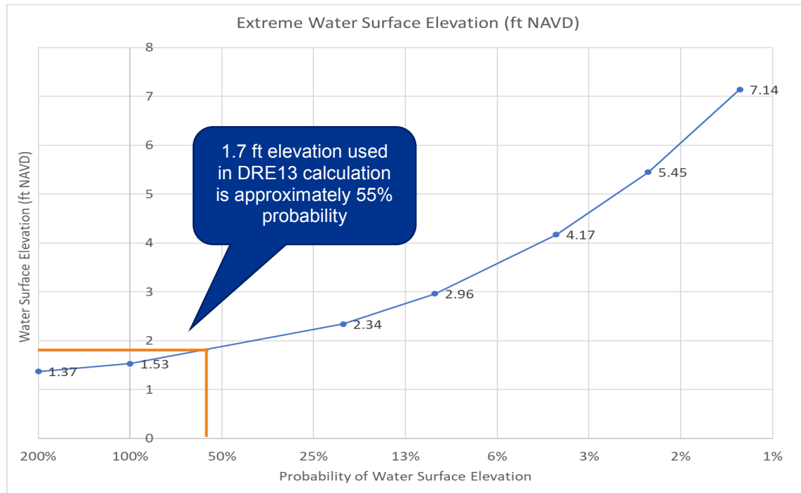
Figure 3. Extreme Value Analysis of Long-Term Water Surface Elevation Data at Virginia Key (1994–2018)
