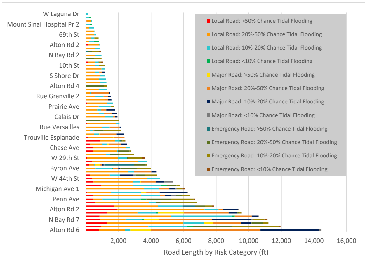
Figure 11. Length of Roads by Type and Flood Risk by Tidal Flood Risk Adaptation Project
