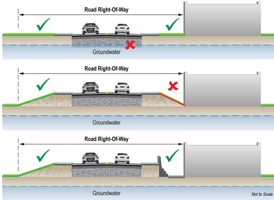
Figure 6. Example of Commercial Property Harmonization
