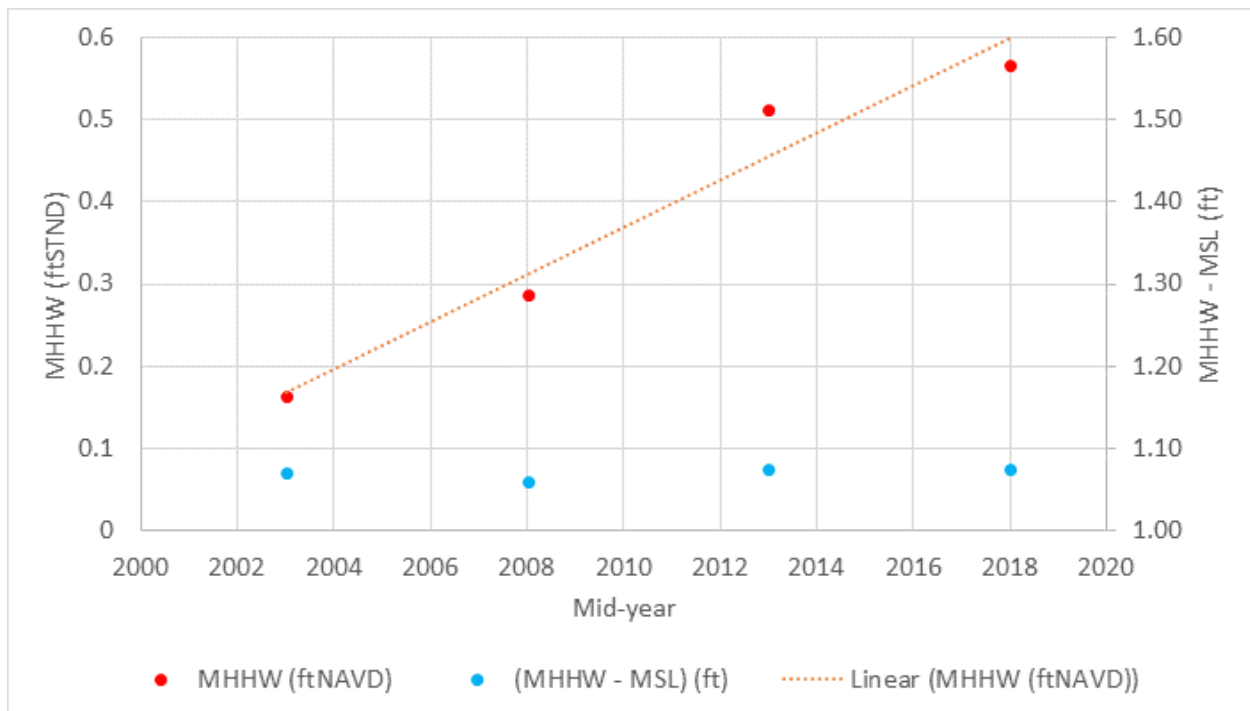
Figure C-1. Variation of MHHW over time, First Method
