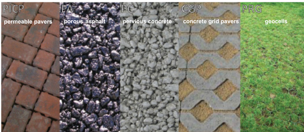
Figure 4. Common Types of Permeable Pavement
