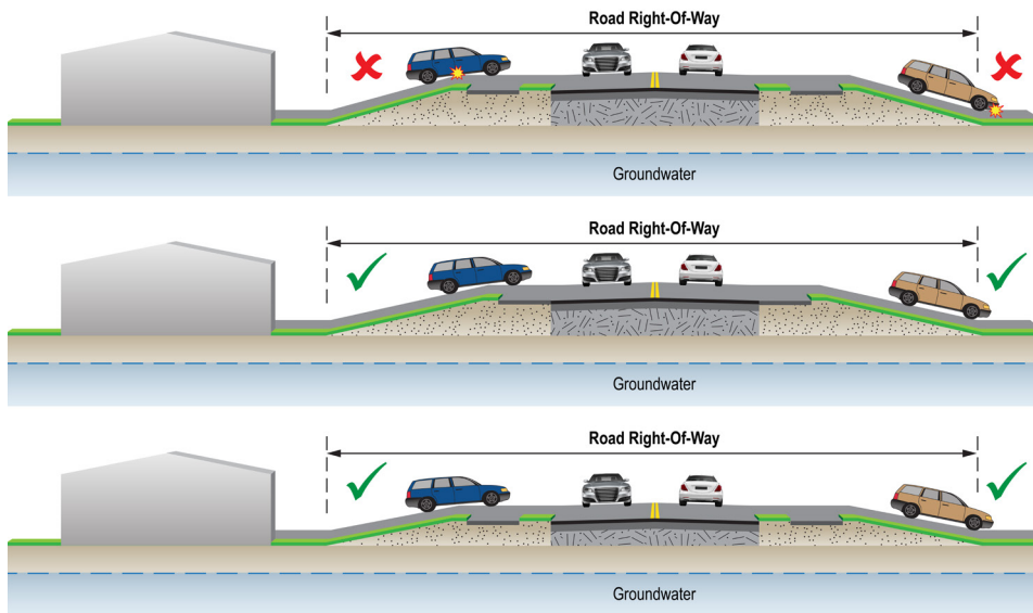
Figure 7. Example of Residential Property Harmonization
