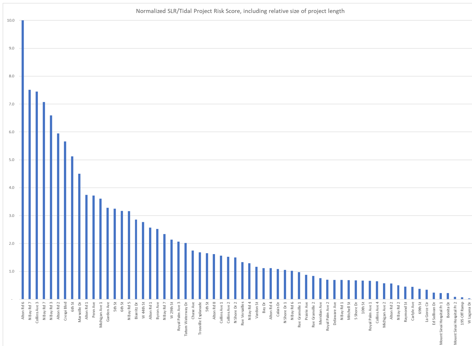
Figure 12. Weighted Risk Score for All Tidal Flood Adaptation Projects, Normalized by Project Total Length
