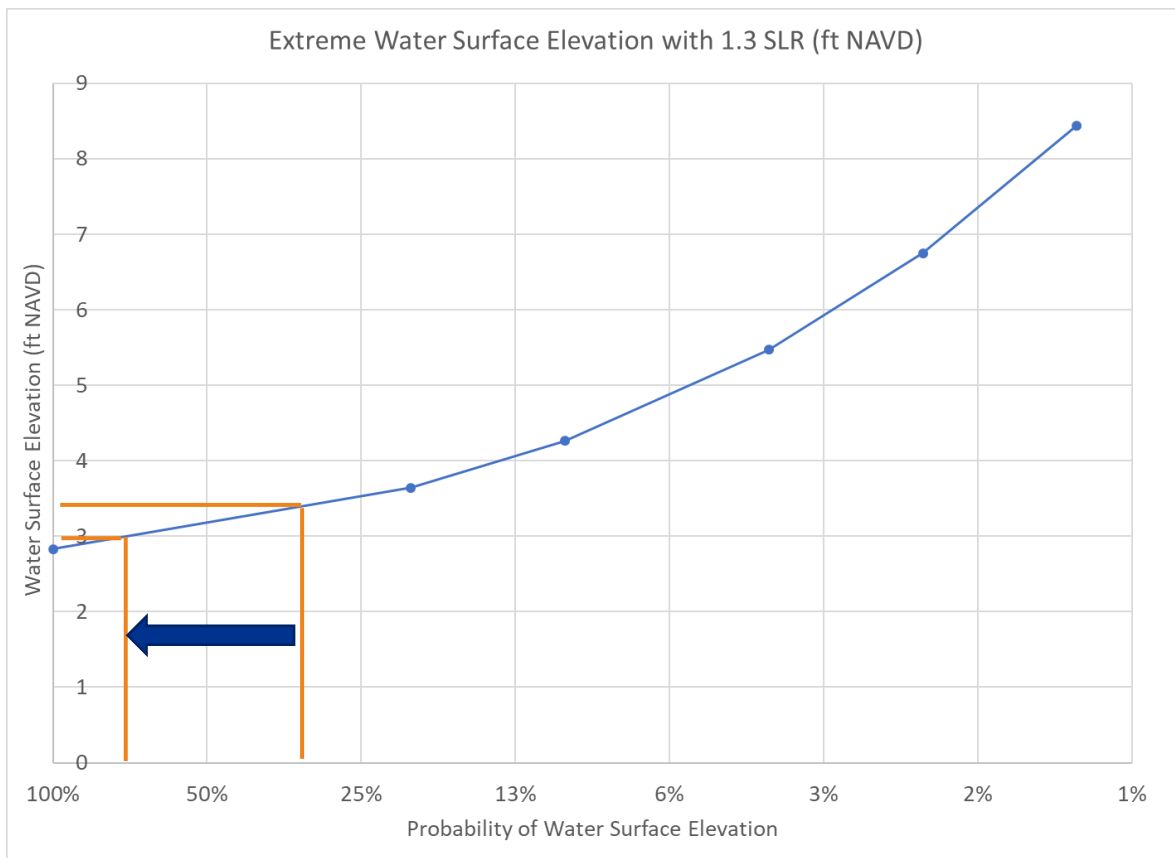
Figure 10. Water Surface Elevations vs. Probability, with Addition of 1.3 ft of SLR
