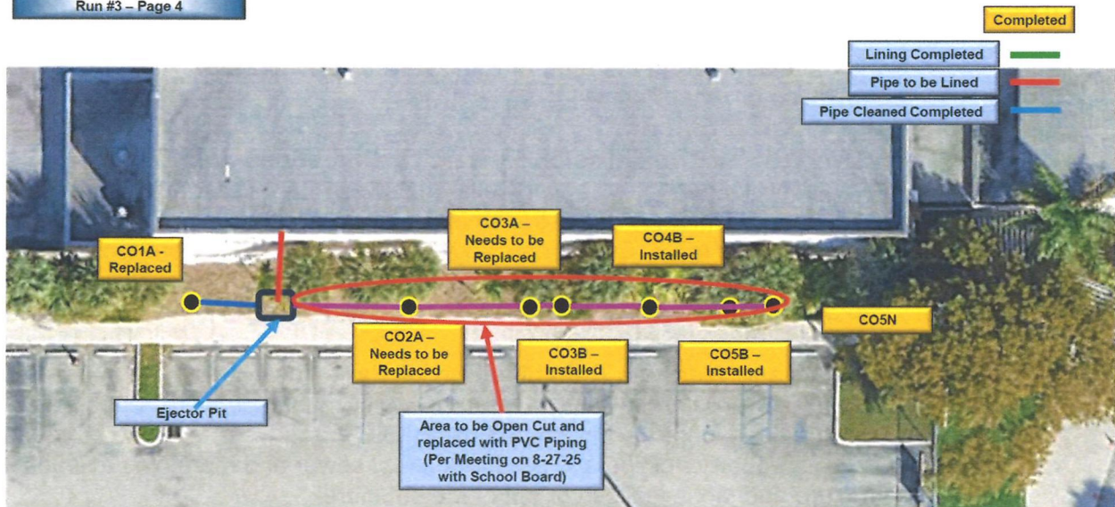
203991-15 – BBE Lateral Lining Run #3 – Page 4
