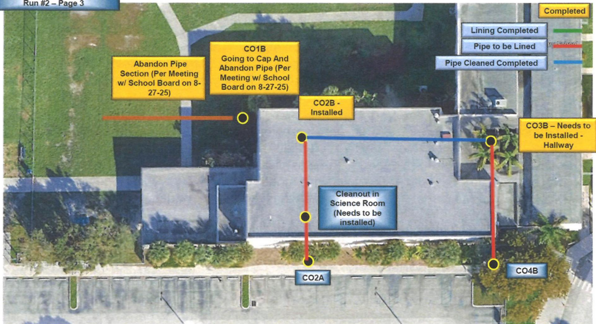
203991-15 – BBE Lateral Lining Run #2 – Page 3
