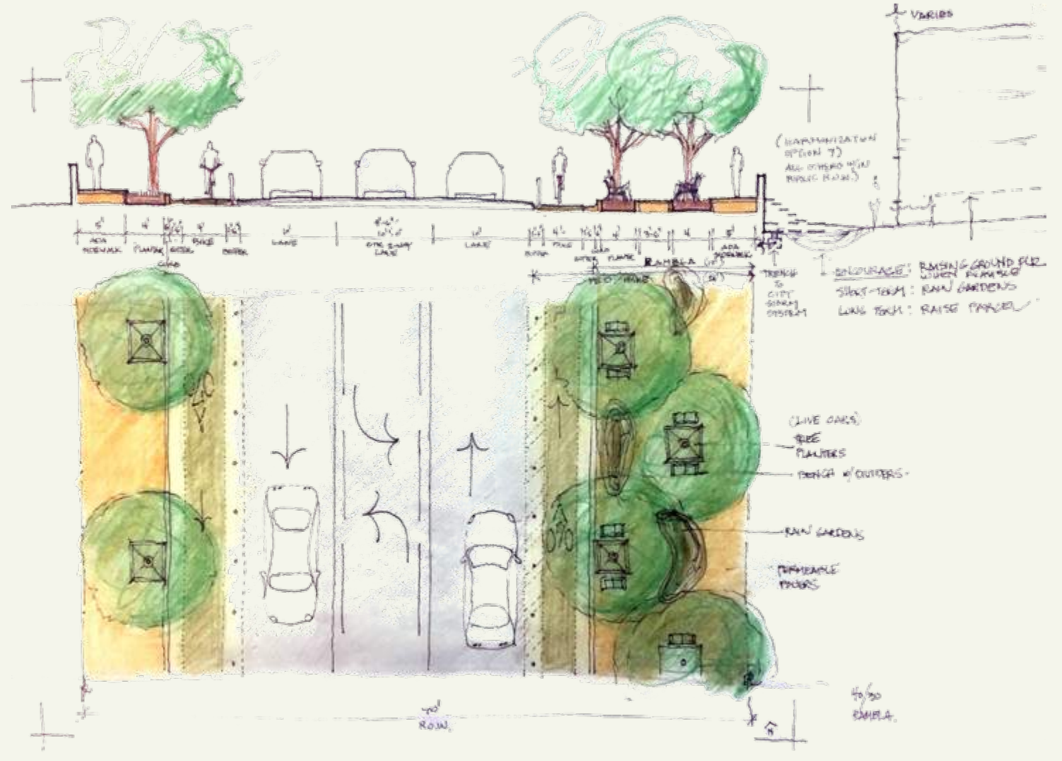
Figure 6.5: Typical section of 8th to 14th Streets delivering intent of Approved Transportation Plan, prioritizing pedestrians and bike lanes - Sonia Chao
